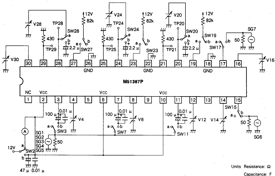
TEST CIRCUIT 2
