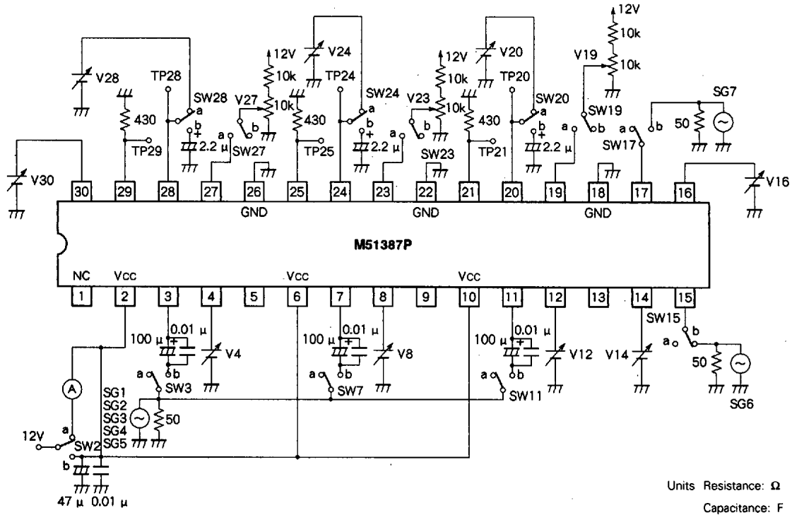
TEST CIRCUIT 1
