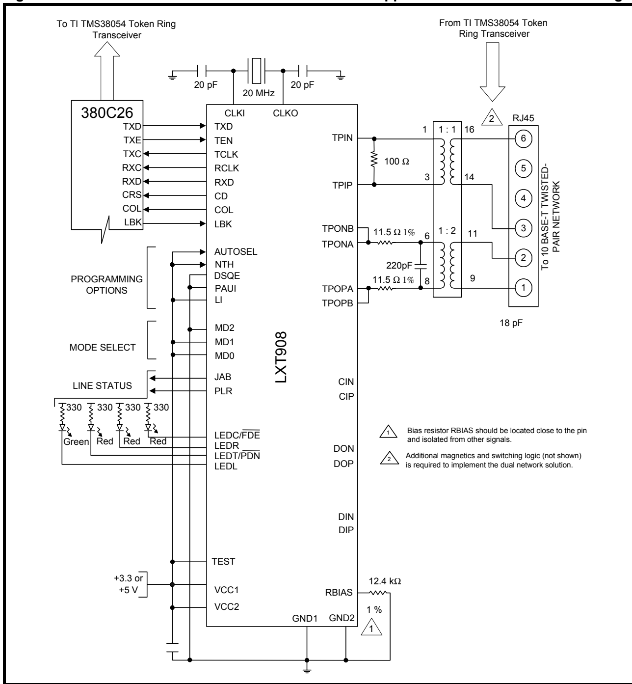
Figure 10: LXT908/380C26 Interface for Dual Network Support of 10BASE-T and Token Ring
