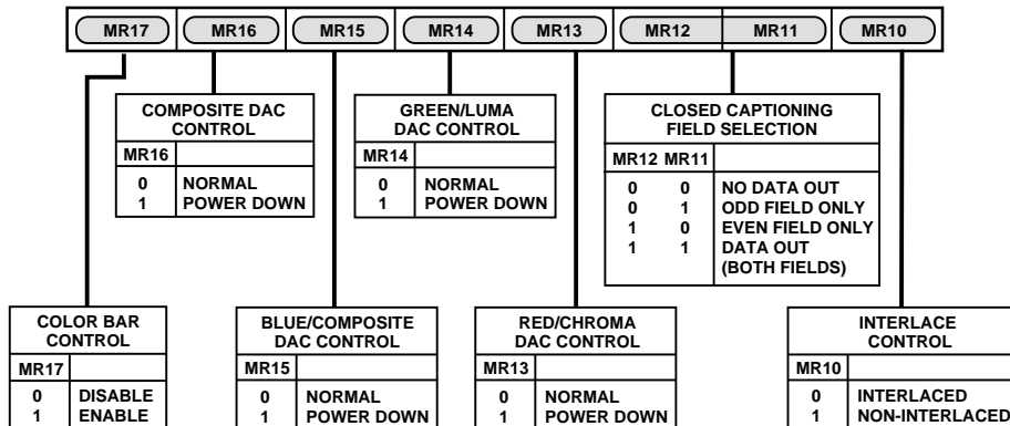
Figure 32. Mode Register 1
