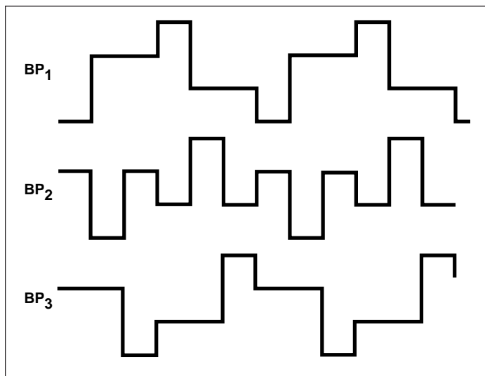
Figure 18. Backplane Waveforms
