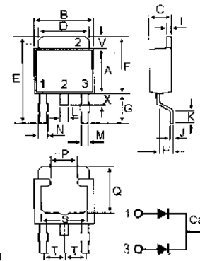
TO-252AA (DPAK)
