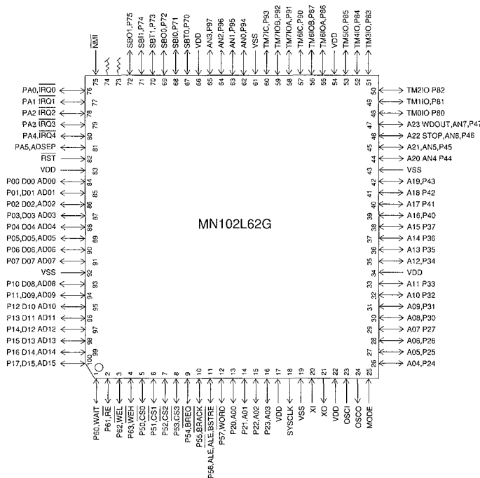
LQFP100-P-1414
