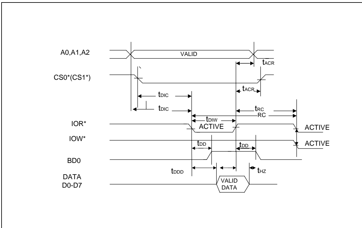
FIGURE 7- Read Cycle Timing
