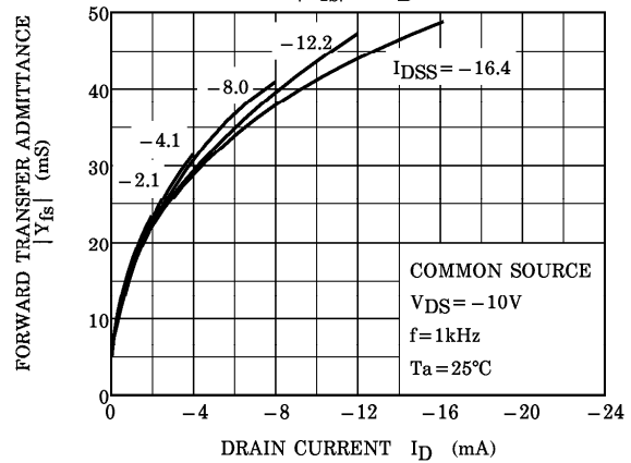
|Yfs| - ID
