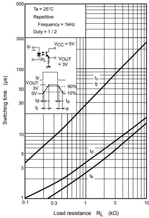
Switching characteristics (non saturated operation) (typ.)
