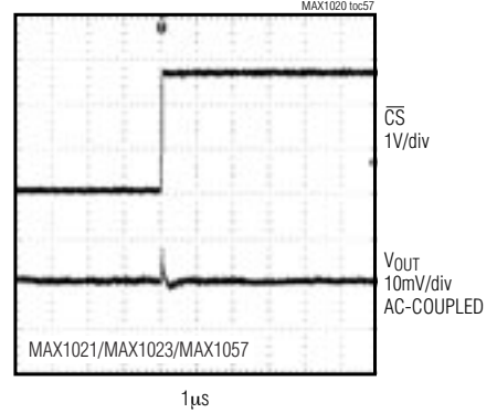
MAJOR CARRY TRANSITION R_{LOAD} = 10k\Omega , C_{LOAD} = 100pF
