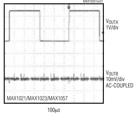
DAC-TO-DAC CROSSTALK R_{LOAD} = 10k\Omega , C_{LOAD} = 100pF
